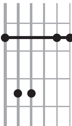
minor
