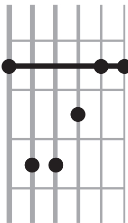
minor
